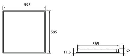
Frida LED 600x600
